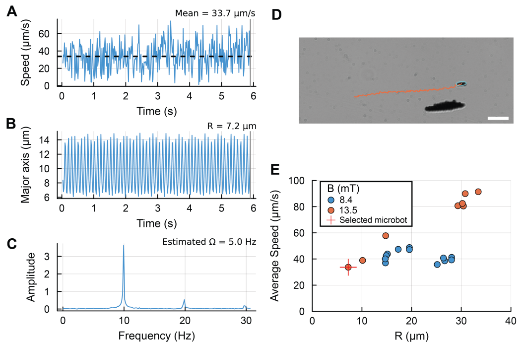
Figure 1: Microbot trajectory analyzer. A) Instantaneous speed and B) major axis of a selected microbot over its lifetime. C) The finite Fourier transform of B enables an estimation of the rotation rate. D) Annotated microscope image of the microbot trajectory and fitted ellipse. Scale = 30 \mu\text{m} . E) Experiment-wide average speed and radius of all microbots and a selected microbot for reference.
